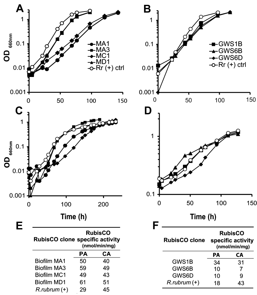
Fig. 3. Autotrophic growth phenotypes and RubisCO activities of enzymes encoded by metagenomic DNA fragments. Anaerobic PA growth (bubbled with 5% CO 2 /95% H 2 ) of: (A) Mono Lake biofilm form I cbbLS fragments; and (B) Rifle groundwater aquifer form II cbbM fragments, each complemented in strain SB I/II. C. Aerobic CA growth (2.5% CO 2 /47.5% H 2 /air) of Mono Lake biofilm form I cbbLS fragments. D. Rifle groundwater aquifer form II cbbM fragments complemented in strain SB I/II- (bubbled with 5% CO 2 /45% H 2 /50% air). Rhodospirillum rubrum cbbM was cloned into plasmid p83 and served as a positive control for complementation of strain SB I/II. Empty vector (p83) served as a negative control (data not shown). RubisCO activities of crude protein lysates of cells harvested from liquid autotrophic cultures that reached an OD of > 1.0 at 660 nm. E. strain SB I/II- expressing Mono Lake biofilm form I RubisCO (encoded by metagenomic cbbLcbbS genes) and (F) strain SB I/II- expressing Rifle groundwater aquifer form II (encoded by metagenomic cbbM gene). The data represent the averages of numbers obtained from two enzyme assay determinations, which both gave similar values.
