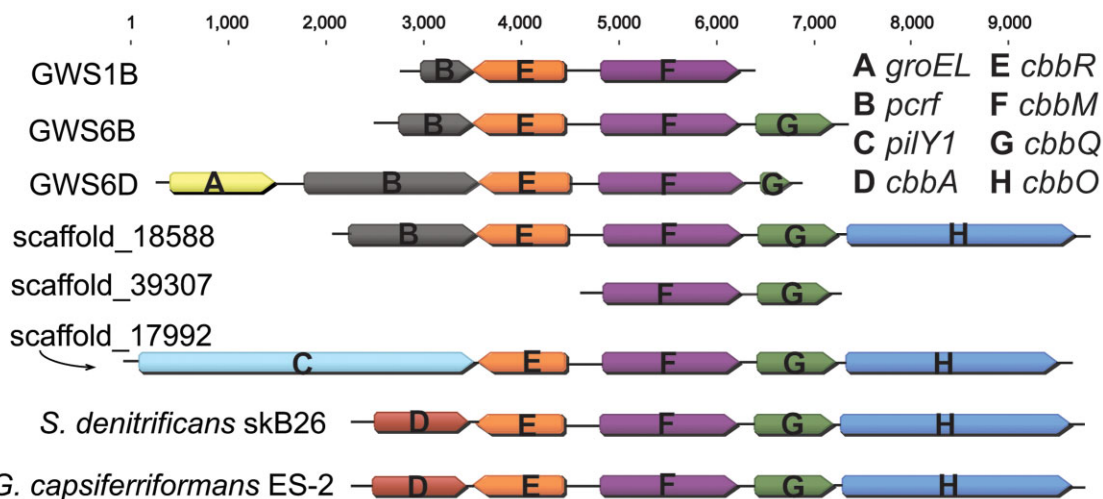
Fig. 4. Operon structure alignments of the recovered metagenomic fragments from the groundwater aquifer. Sequences are from the Rifle groundwater aquifer, along with closest RubisCO hits and related sequences available in the NCBI database. The acronym pcrf stands for peptide chain release factor.
