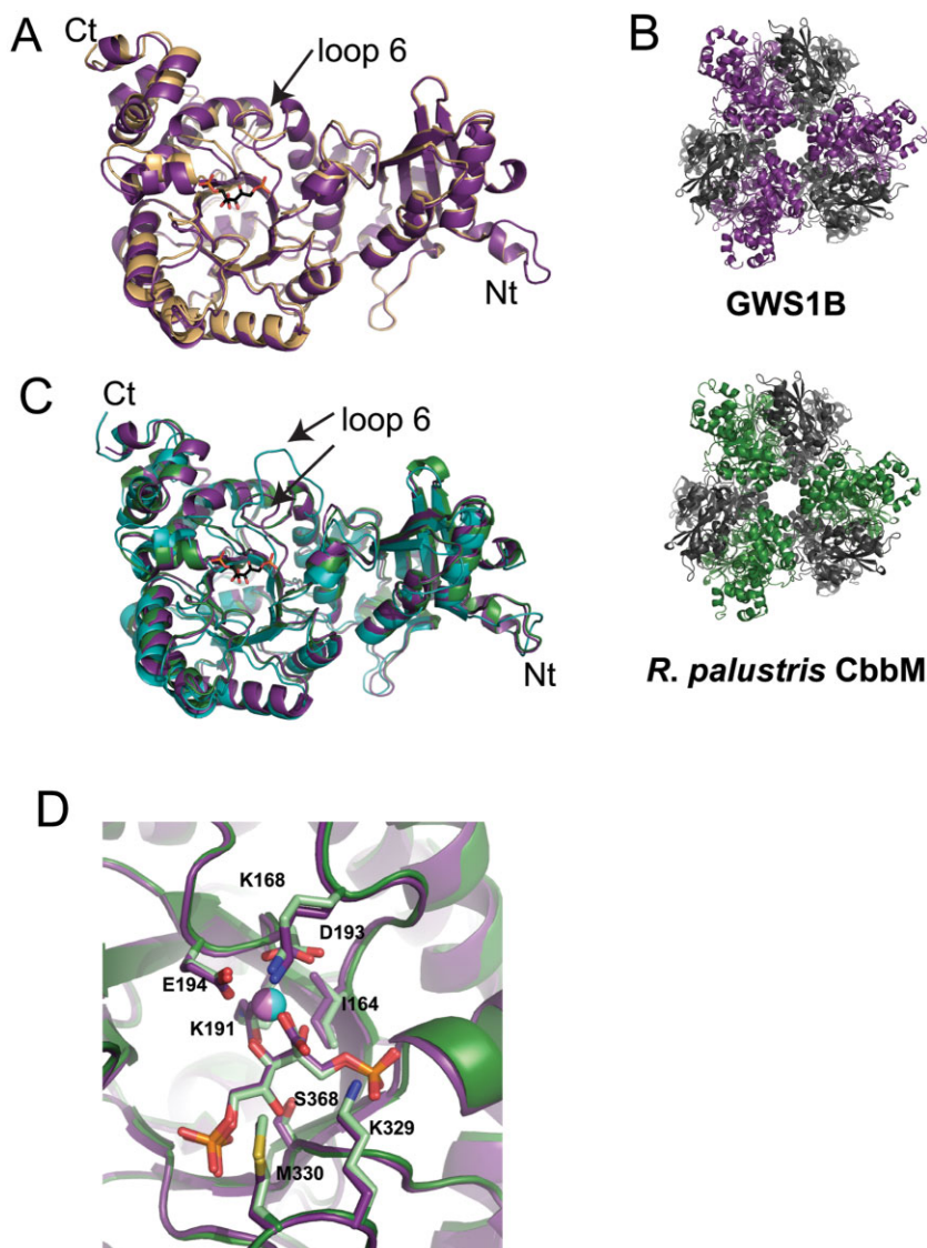
Fig. 5. Structural characteristics of form II RubisCO (GWS1B) from uncultivated Gallionellaceae species.
