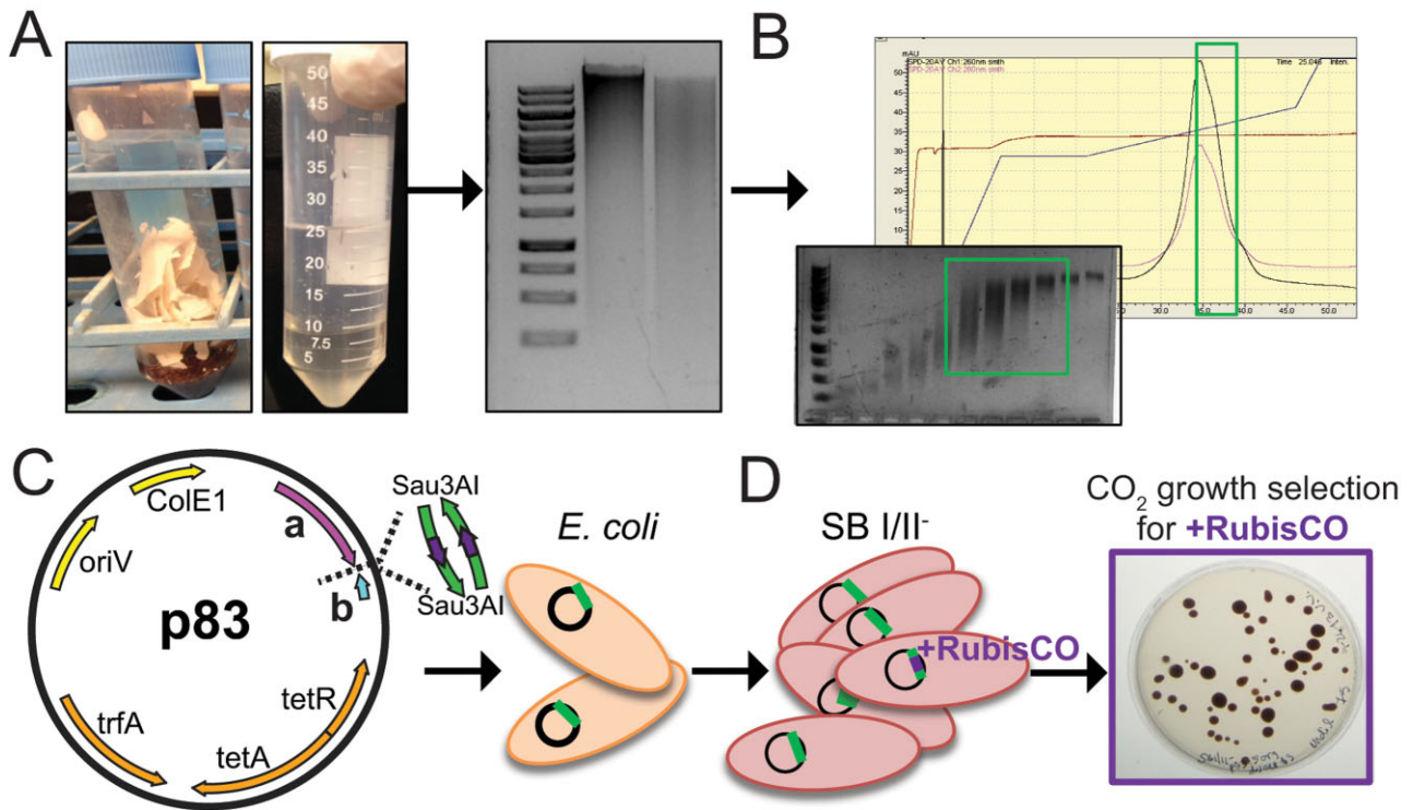
Fig. 1. Selection approach to recover functional metagenomic RubisCO sequences.
