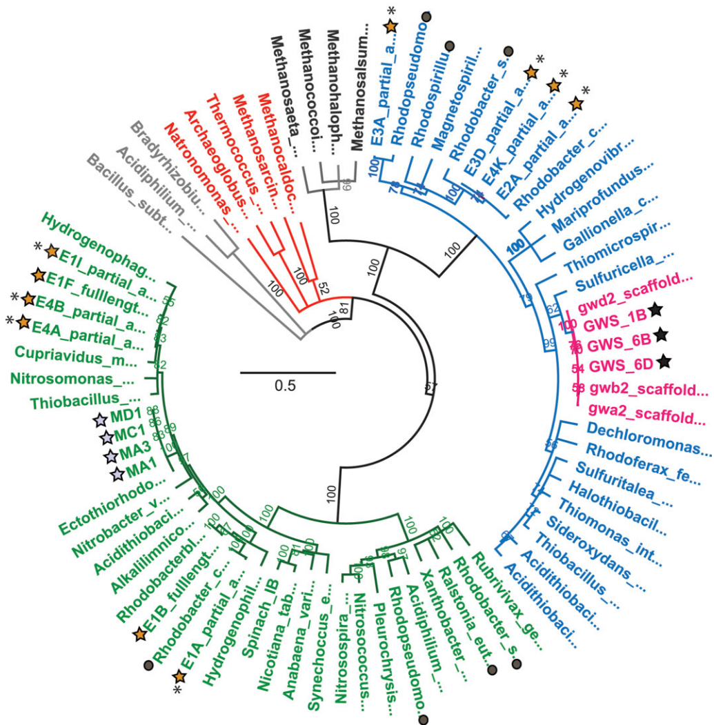
Fig. 2. RubisCO amino-acid tree of functionally selected RubisCOs. The following colour scheme was used: RubisCO form I sequences (green), form II (blue), form II Gallionellaceae (pink), hybrid form II/III (black), form III (red), and form IV (gray). Sequences retrieved as part of this study are marked with a star filled with various colours identifying the nature of the strain: Enrichment (orange), Biofilm (gray), and Groundwater aquifer (black). RubisCO sequences employed as part of the five-organism control experiment are indicated by gray-filled circles. Enrichment RubisCO sequences noted with asterisks are partial sequences encompassing aa 130–458 according to R. rubrum numbering for the form II and aa 80–410 according to Synechococcus PCC6301 numbering for the form I sequences. The rest of the sequences are full-length RubisCO sequences. Representative full-length RubisCO sequences were obtained from the NCBI ref seq database (Table S1). The distance-based RubisCO amino acid tree was made in GENEIOUS using the Jukes-Cantor genetic distance model and the neighbour-joining tree building method. Bacillus subtilis form IV RubisCO served as the outgroup. The tree was re-sampled using bootstrapping with 100 replicates.
