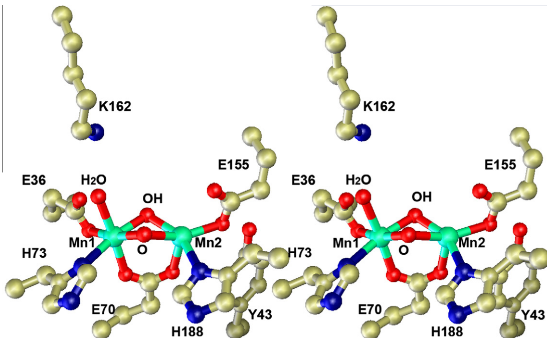
Fig. 7. Active site of native Mn(III,III) Thermus thermophilus manganese catalase. Stereoscopic view of the binuclear manganese complex in the oxidized Mn 2 (III,III) state. Based on PDB ID: 2V8U.
