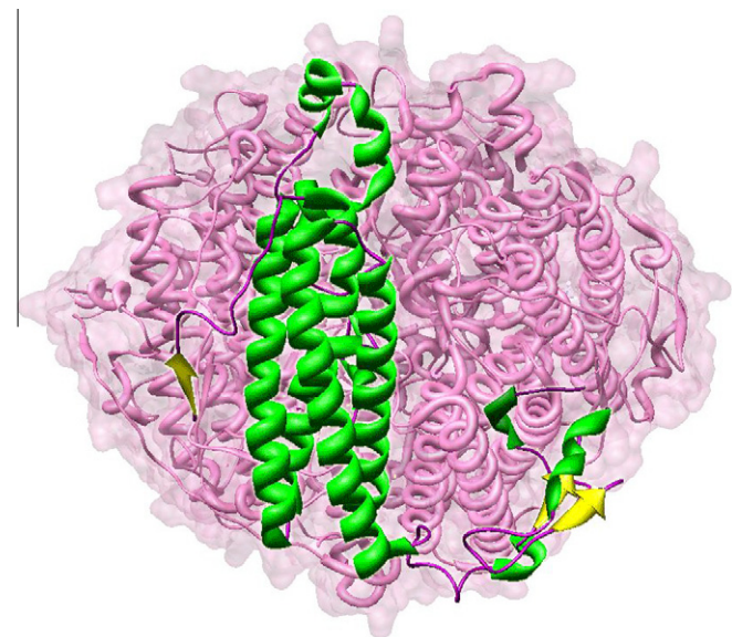
Fig. 1. Lactobacillus plantarum manganese catalase. A single subunit of LPC is rendered as ribbons embedded in the surface-rendered globular hexameric holoenzyme. Based on PDB ID: 1JKU.
