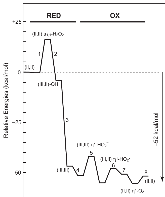
Fig. 10. Manganese catalase turnover reaction energy profile. (Based on Ref. [37].)
