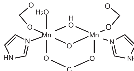
Fig. 9. Active site model used for ab initio calculation of reaction energy profile. (Based on Ref. [37].)
