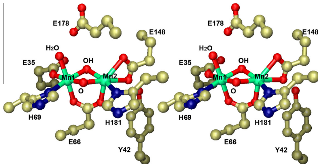
Fig. 3. Active site of native Mn(III,III) Lactobacillus plantarum manganese catalase. Stereoscopic view of the binuclear manganese complex in the oxidized Mn 2 (III,III) state. Based on PDB ID: 1JKU.
