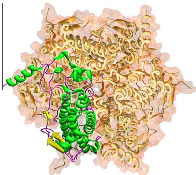
Fig. 6. Thermus thermophilus manganese catalase. A single subunit of TTC is rendered as ribbons embedded in the surface-rendered globular hexameric holoenzyme. Based on PDB ID: 2V8U.
