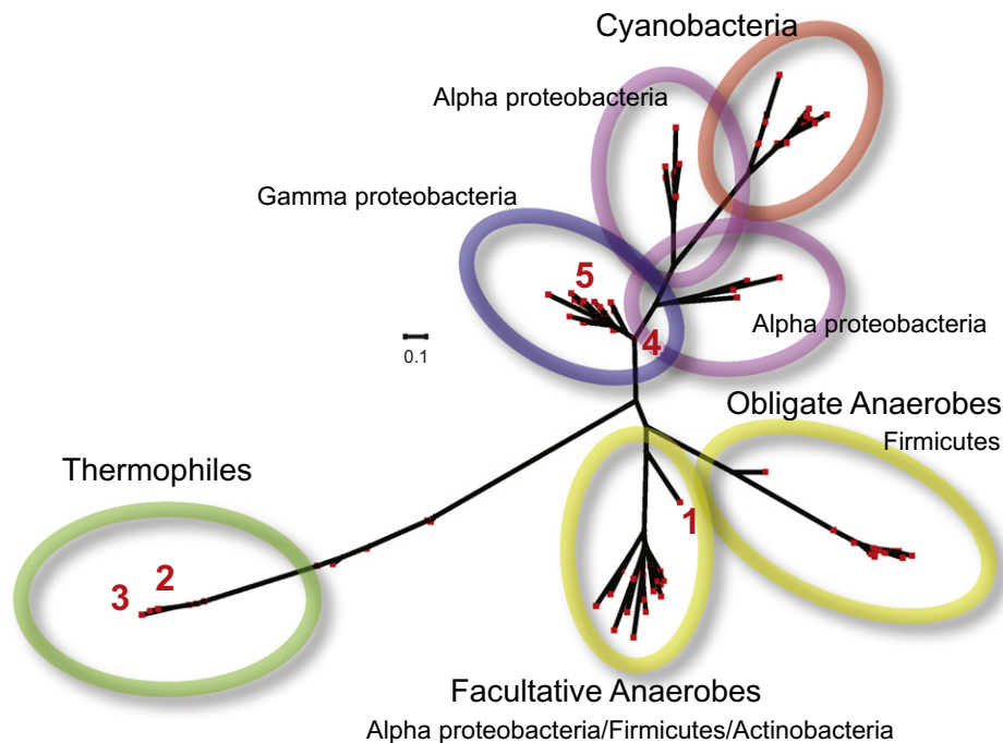
Fig. 11. Radial phylogenetic tree for putative manganese catalases in genomic databases. (1) Lactobacillus plantarum manganese catalase (LPC); (2) Thermus thermophilus manganese catalase (TTC); (3) Pyrobaculum caldifontis manganese catalase; (4) Salmonella enterica katNp; (5) Escherichia coli O157:H7 Z1921p. Generated from the predicted protein sequences using Phylip cluster analysis [42] and Dendroscope-3 tree builder [43].
