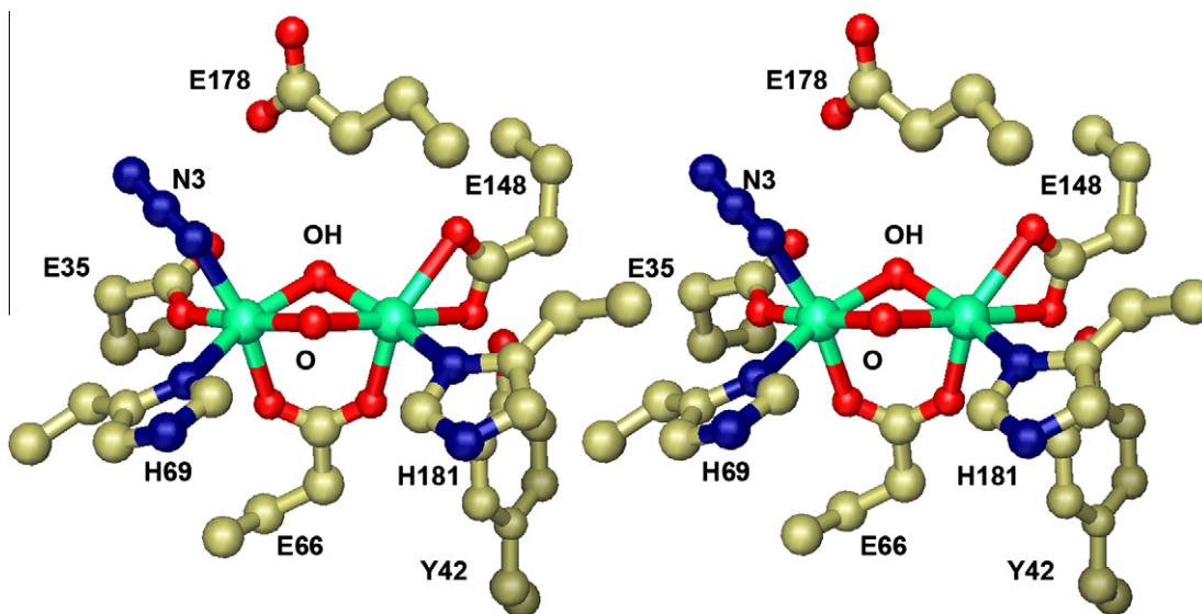
Fig. 4. Active site of azide-bound Lactobacillus plantarum manganese catalase. Stereoscopic view of the binuclear manganese complex in the oxidized Mn_2(III,III) state with azide bound. Based on PDB ID: 1JKV.
