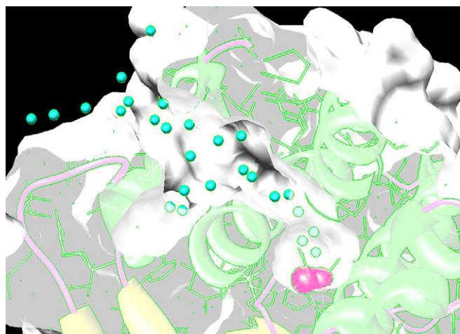
Fig. 8. The 22 Å long access channel in TTC. A cross-section of the TTC four-helix bundle is shown, near the level of the binuclear manganese active site (red spheres). The protein is surface-rendered and solvent molecules within the channel appear as cyan spheres. Based on PDB ID: 2V8U.
