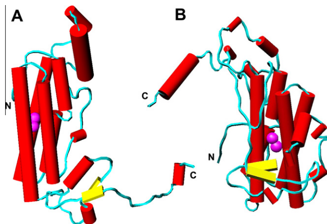
Fig. 2. Structure of manganese catalase subunits. Secondary structural elements of (A) LPC (based on PDB ID: 1JKU) and (B) TTC (based on PDB ID: 2V8U) polypeptides is indicated: \alpha -helix, red; \beta -sheet, yellow; turn, blue. Manganese ions are rendered as magenta spheres. N- and C-terminal regions are noted.
