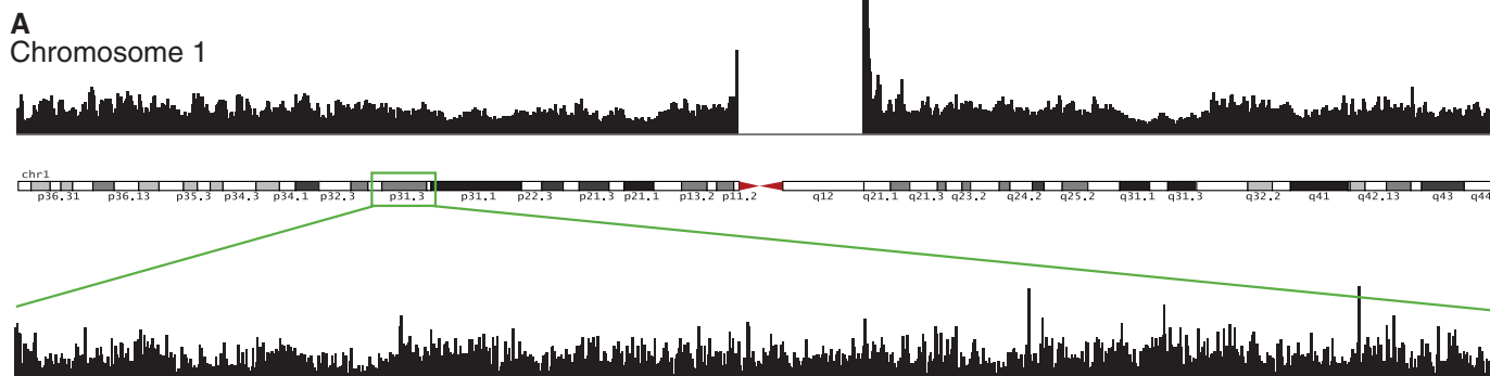
Fig. 2. Characterization of amplification uniformity. (A) Histograms of reads over the entirety of chromosome 1 (chr1) of a single cell from the SW480 cancer cell line and the zoom-in of an ~8-million-base region (chr1: 62,023,147 to 70,084,845). (B) Lorenz curves of MALBAC, MDA, and the bulk sample. A Lorenz curve gives the cumulative fraction of reads as a function of the cumulative fraction of genome. Perfectly uniform coverage would result in a diagonal line, and a large deviation from the diagonal is indicative of biased coverage. The blue and green arrows indicate the uncovered fractions of the genome for MALBAC and MDA, respectively. All samples are sequenced at 25x depth. (C) Power spectrum of read density throughout the genome (as a function of spatial frequency). MALBAC performs similarly to bulk, whereas the MDA spectrum shows high amplitude at low frequency, demonstrating that regions of several megabases suffer from under- and overamplification. This observation is consistent with the variations of read depth in fig. S3.
