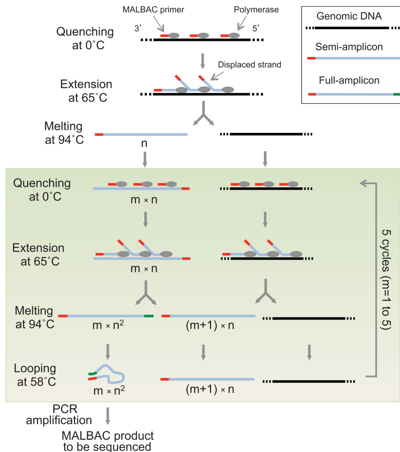
Fig. 1. MALBAC single-cell whole-genome amplification. A single cell is picked and lysed. First, genomic DNA of the single cell is melted into single-stranded DNA molecules at 94°C. MALBAC primers then anneal randomly to single-stranded DNA molecules at 0°C and are extended by a polymerase with displacement activity at elevated temperatures, creating semiamplicons. In the following five temperature cycles, after the step of looping the full amplicons, single-stranded amplicons and the genomic DNA are used as a template to produce full amplicons and additional semiamplicons, respectively. For full amplicons, the 3' end is complementary to the sequence on the 5' end. The two ends hybridize to form looped DNA, which can efficiently prevent the full amplicon from being used as a template, therefore warranting a close-to-linear amplification. After the five cycles of linear preamplification, only the full amplicons can be exponentially amplified in the following PCR using the common 27-nucleotide sequence as the primer. PCR reaction will generate microgram level of DNA material for sequencing experiments.
