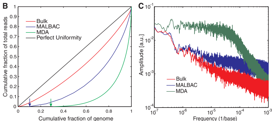
Fig. 2. Characterization of amplification uniformity. (A) Histograms of reads over the entirety of chromosome 1 (chr1) of a single cell from the SW480 cancer cell line and the zoom-in of an ~8-million-base region (chr1: 62,023,147 to 70,084,845). (B) Lorenz curves of MALBAC, MDA, and the bulk sample. A Lorenz curve gives the cumulative fraction of reads as a function of the cumulative fraction of genome. Perfectly uniform coverage would result in a diagonal line, and a large deviation from the diagonal is indicative of biased coverage. The blue and green arrows indicate the uncovered fractions of the genome for MALBAC and MDA, respectively. All samples are sequenced at 25x depth. (C) Power spectrum of read density throughout the genome (as a function of spatial frequency). MALBAC performs similarly to bulk, whereas the MDA spectrum shows high amplitude at low frequency, demonstrating that regions of several megabases suffer from under- and overamplification. This observation is consistent with the variations of read depth in fig. S3.
