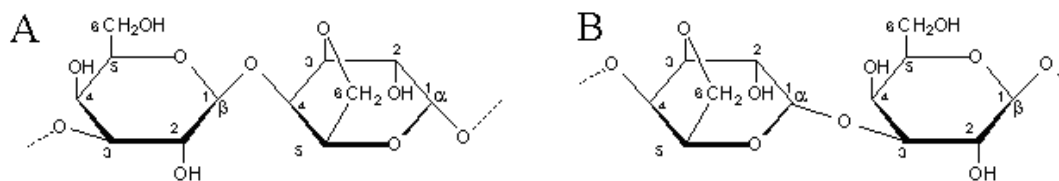
Figure 2. Structure of agarobiose (A) and neoagarobiose (B).
