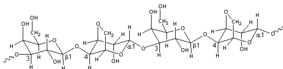
Figure 1. Structure of agarose.
