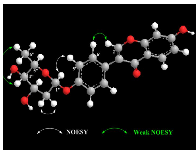
Figure 4. The key NOESY correlations for compound 1.
