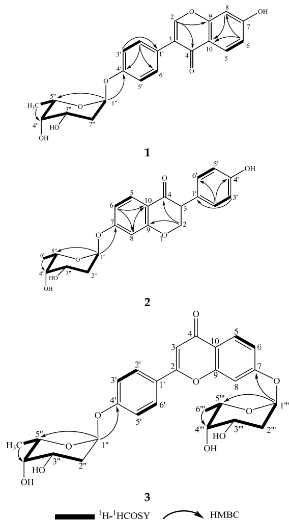
Figure 3. The structures and key ^1\text{H} - ^1\text{H} COSY and HMBC correlations for compounds 1–3.
