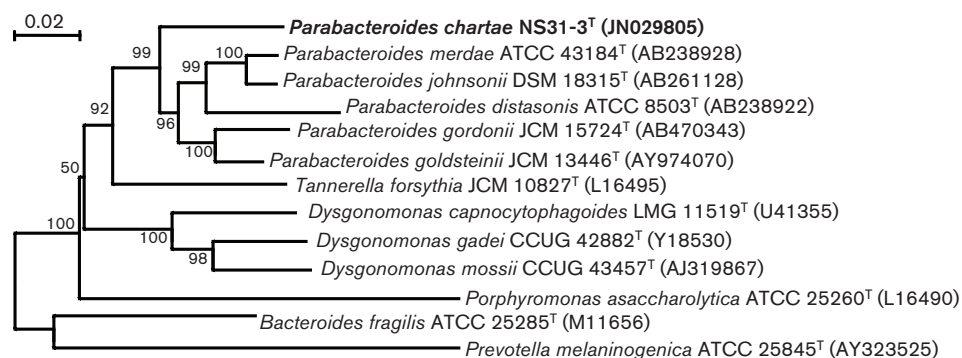
Fig. 1. Neighbour-joining phylogenetic tree based on 16S rRNA gene sequences, showing the phylogenetic relationships of strain NS31-3 T and related taxa. Bootstrap values (≥50%) based on 1000 replicates are shown at branch nodes. Bar, 0.02 substitutions per nucleotide position.
